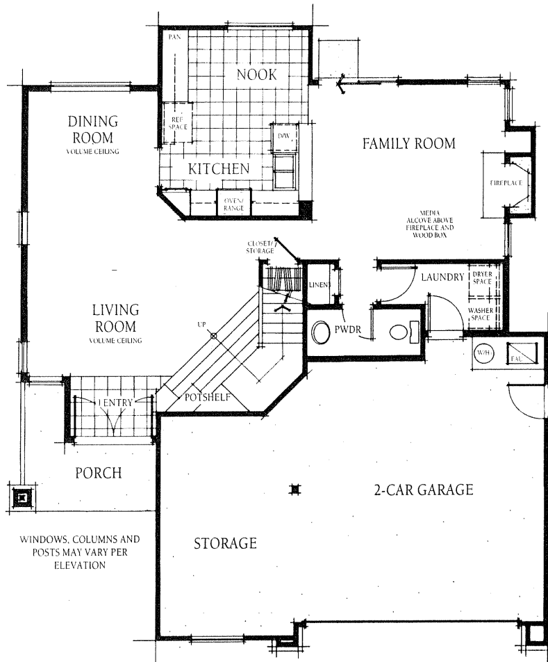
FIRST FLOOR
